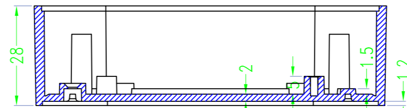
SEC B-B
