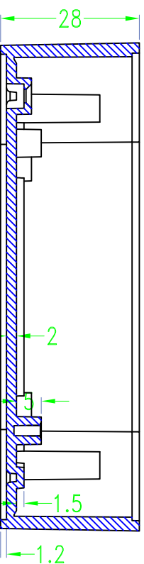
SEC B-B
