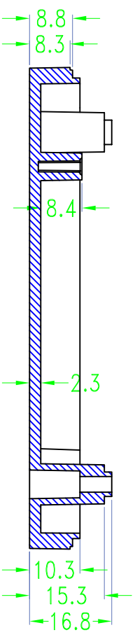
SEC C-C
