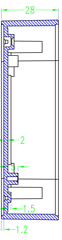
SEC B-B
