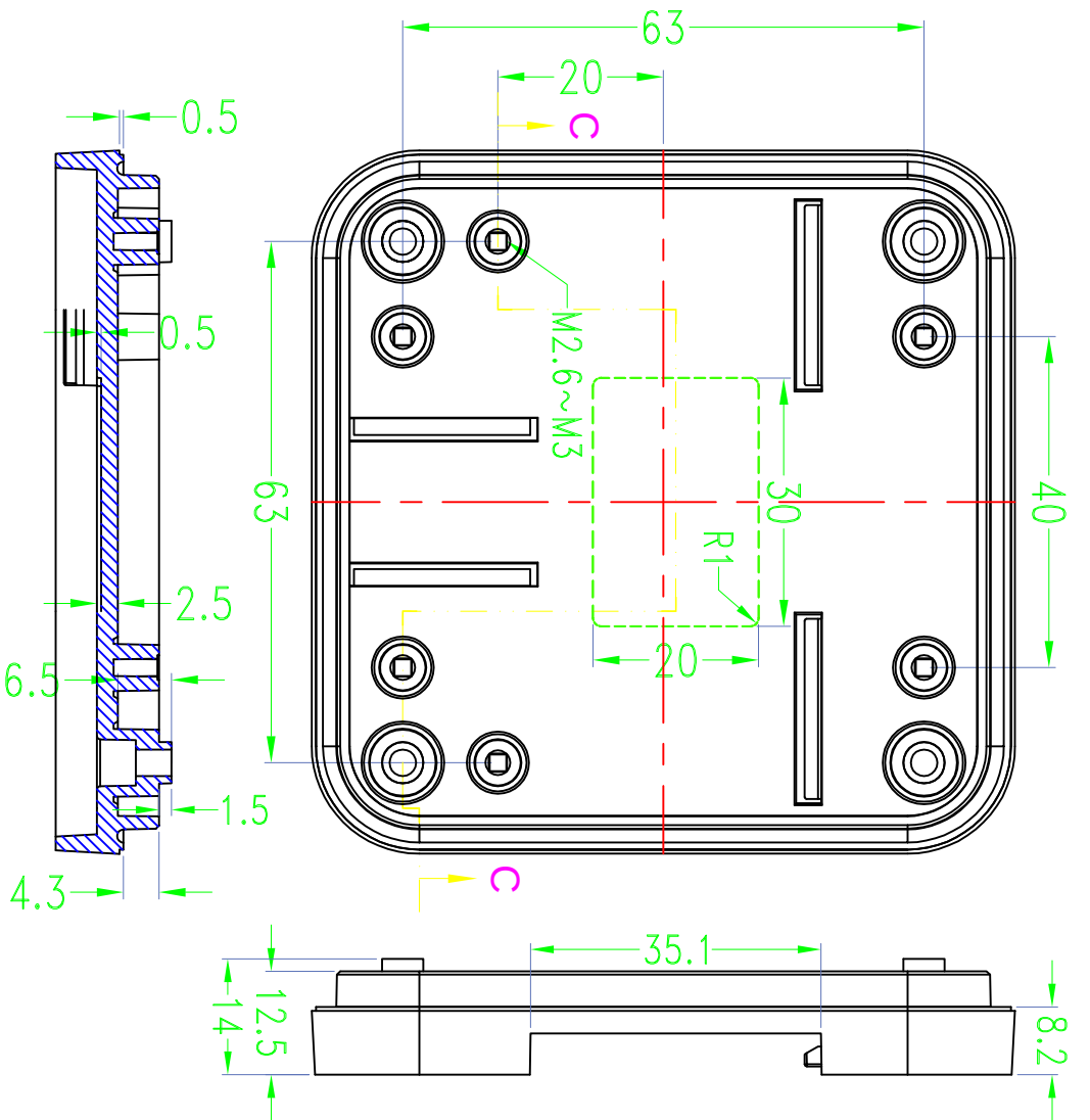
SEC C-C
