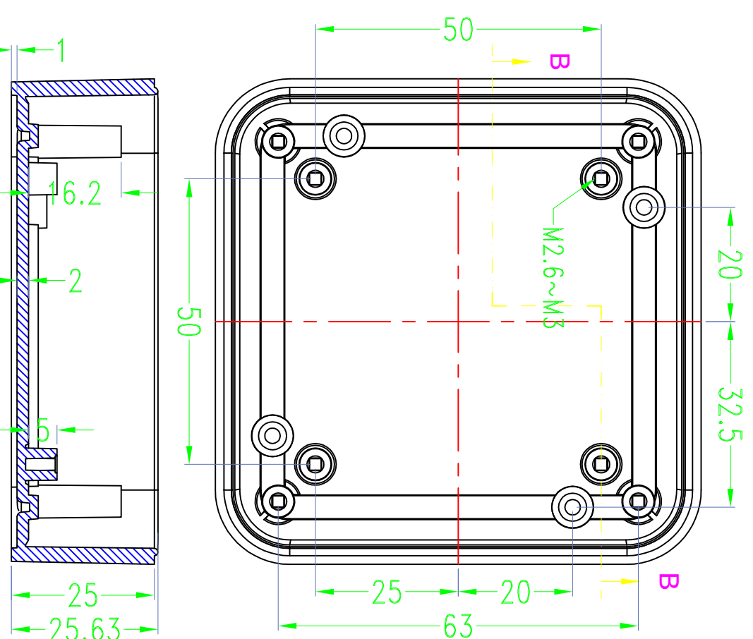
SEC B-B
