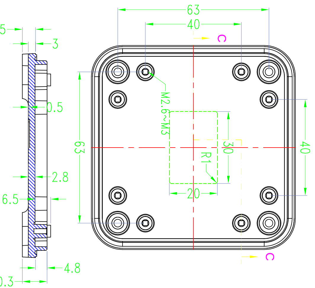
SEC C-C
