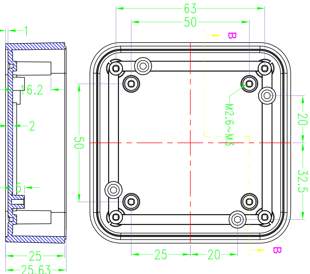
SEC B-B
