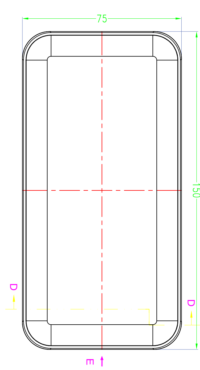
SEC C-C
