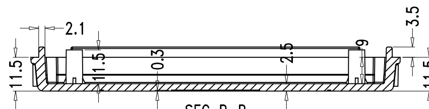
SEC B-B
