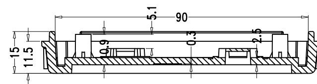
SEC B-B
