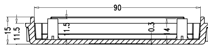
SEC B-B
