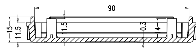
SEC B-B
