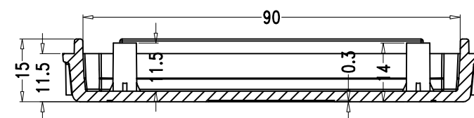
SEC B-B
