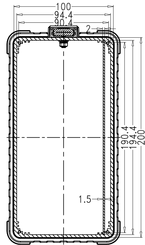
SEC B-B
