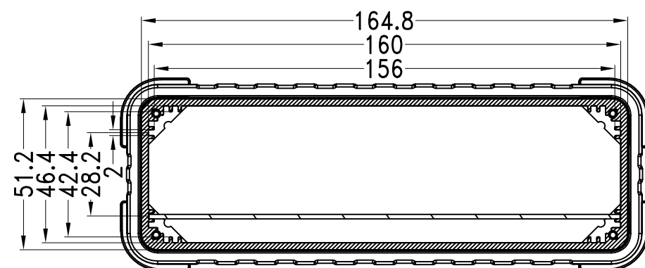
SEC B-B
