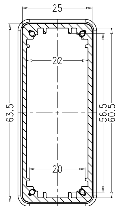
SEC B-B
