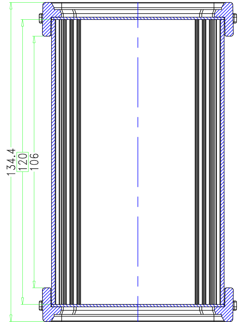
SEC B-B
