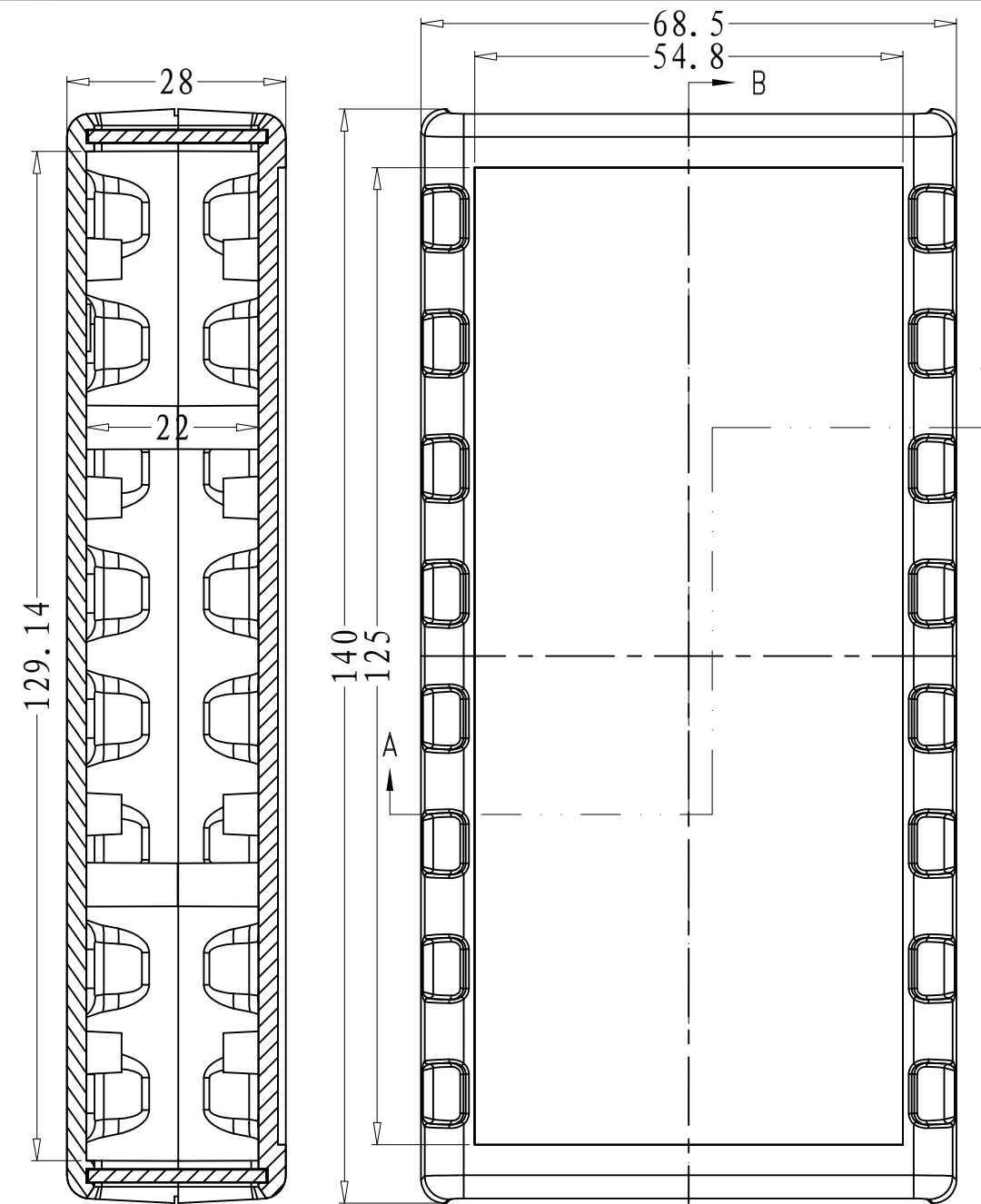
SEC B-B
