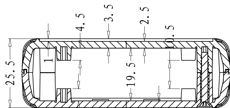
SEC B-B
