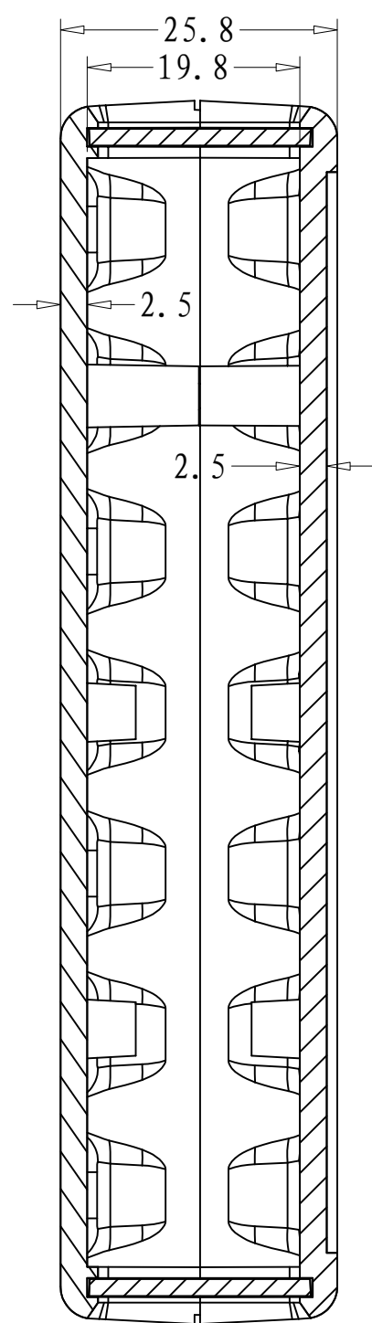
SEC B-B
